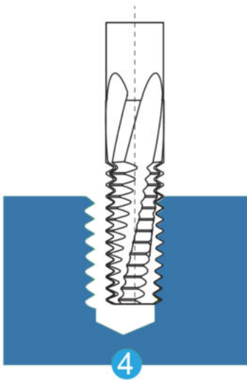
4 360° Spiral Machining
