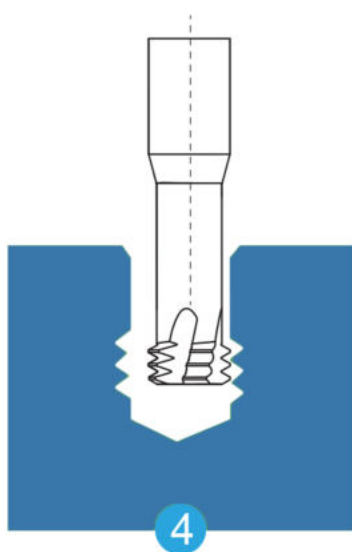
4 Continue Process Upward until Thread is Complete
