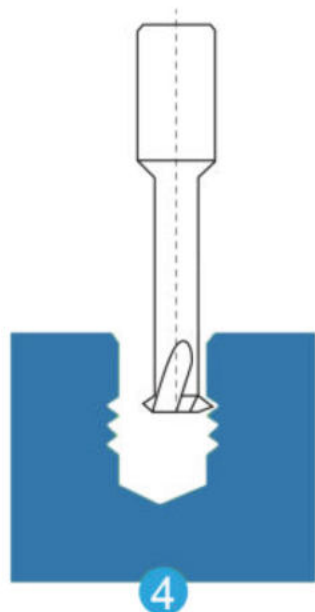
4 Continue Process Upward until Thread is Complete
