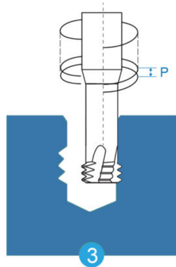
3 Feed to Arc on Position, Spiral Feed acc. to Thread Pitch
