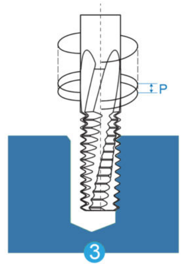
3 Feed to Arc on Position and Spiral Feed for One Pitch
