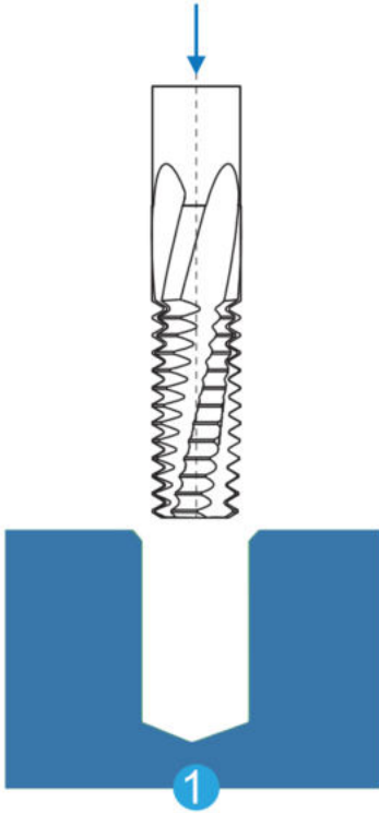
1 Position above Hole Center
